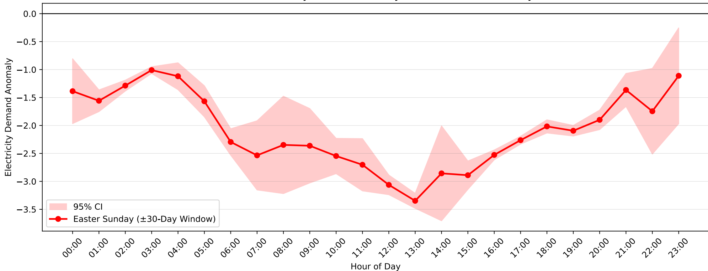
Cardiff Demand Anomaly: Easter Sunday (2014-2015, \pm 30 -Day Window)
