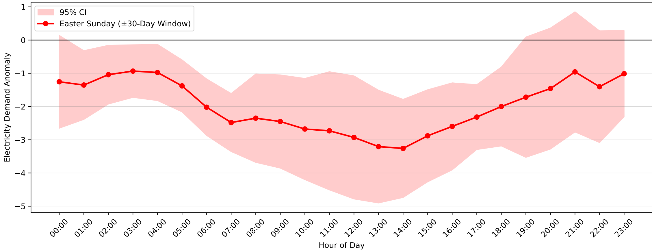
Cardiff Demand Anomaly: Easter Sunday (2016–2017, \pm 30 -Day Window)
