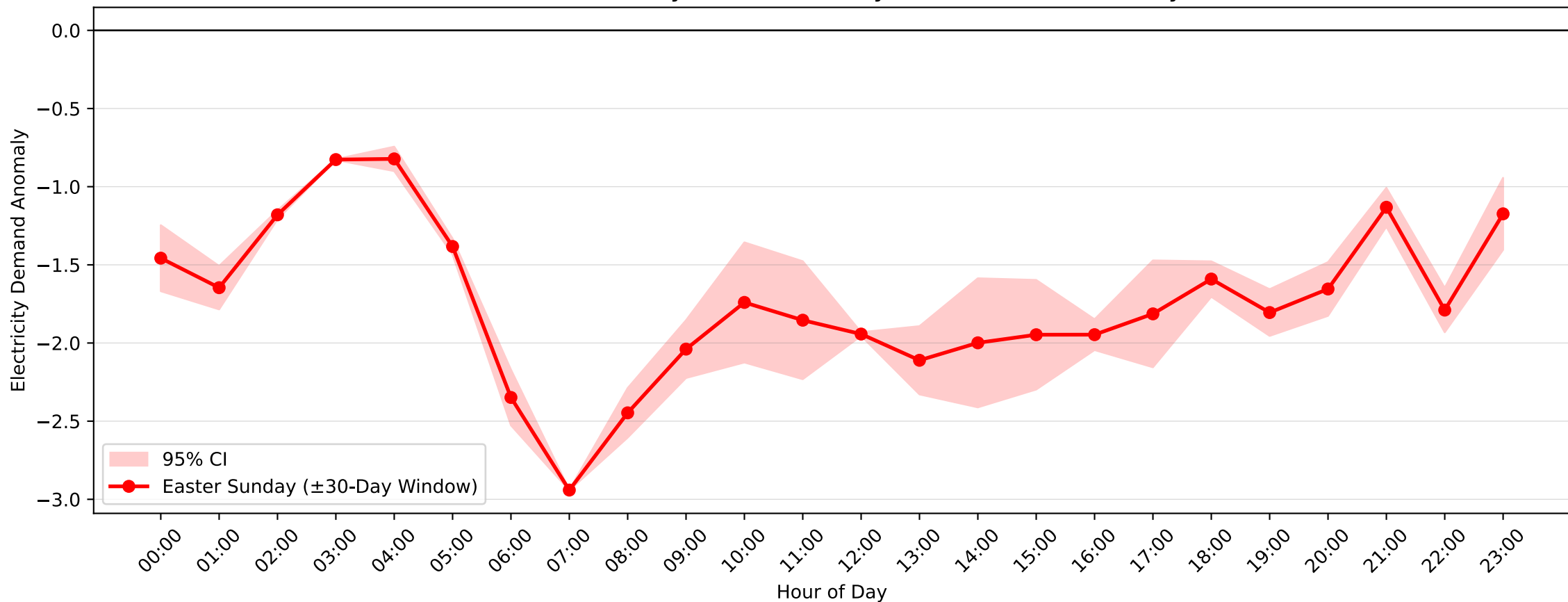
Cardiff Demand Anomaly: Easter Sunday (2011-2012, \pm 30 -Day Window)
