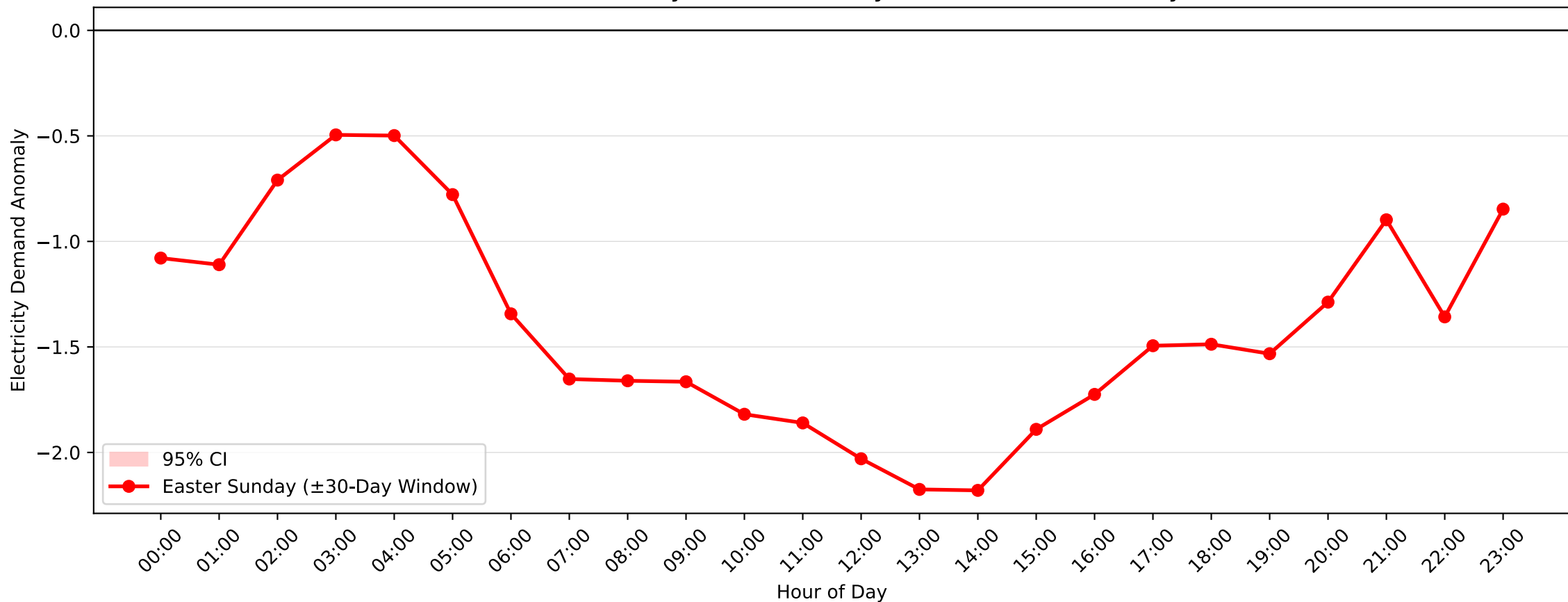
Cardiff Demand Anomaly: Easter Sunday (2017-2018, \pm 30 -Day Window)
