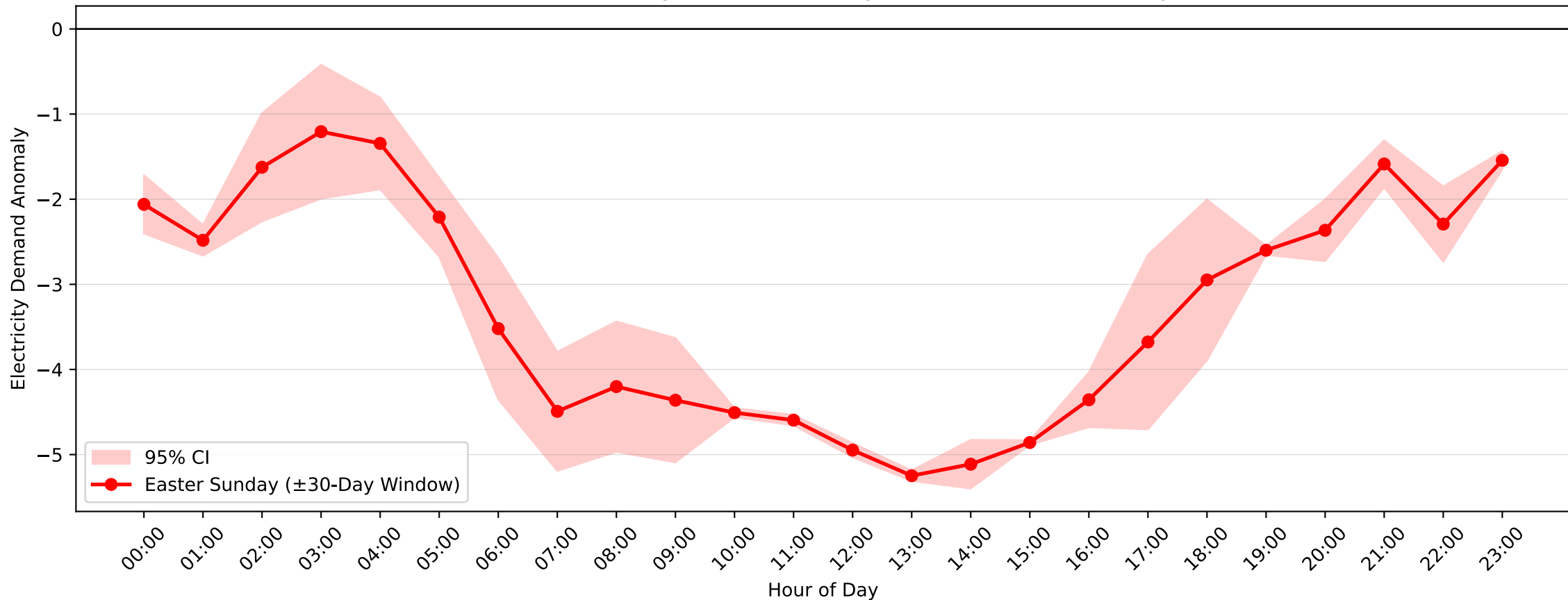
Cardiff Demand Anomaly: Easter Sunday (2008–2009, \pm 30 -Day Window)
